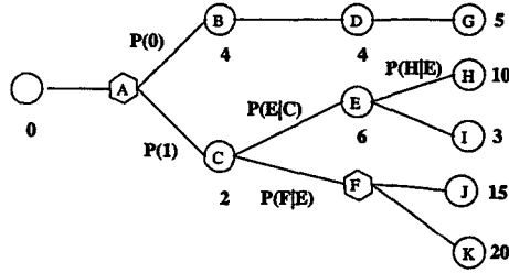
Figure 1: An agent's stochastic performance profile tree for a valuation problem. The hexagonal nodes are random nodes and the round nodes are value nodes. At random node A, the probability that the random number will be 0 is P(0) , and the probability that the random number will be 1 is P(1) . The edges from any value node have a weight of one time step, while the edges from any random node have a weight of zero time steps. This means it takes 3 time steps to reach node G, and 2 time steps to reach node J.
